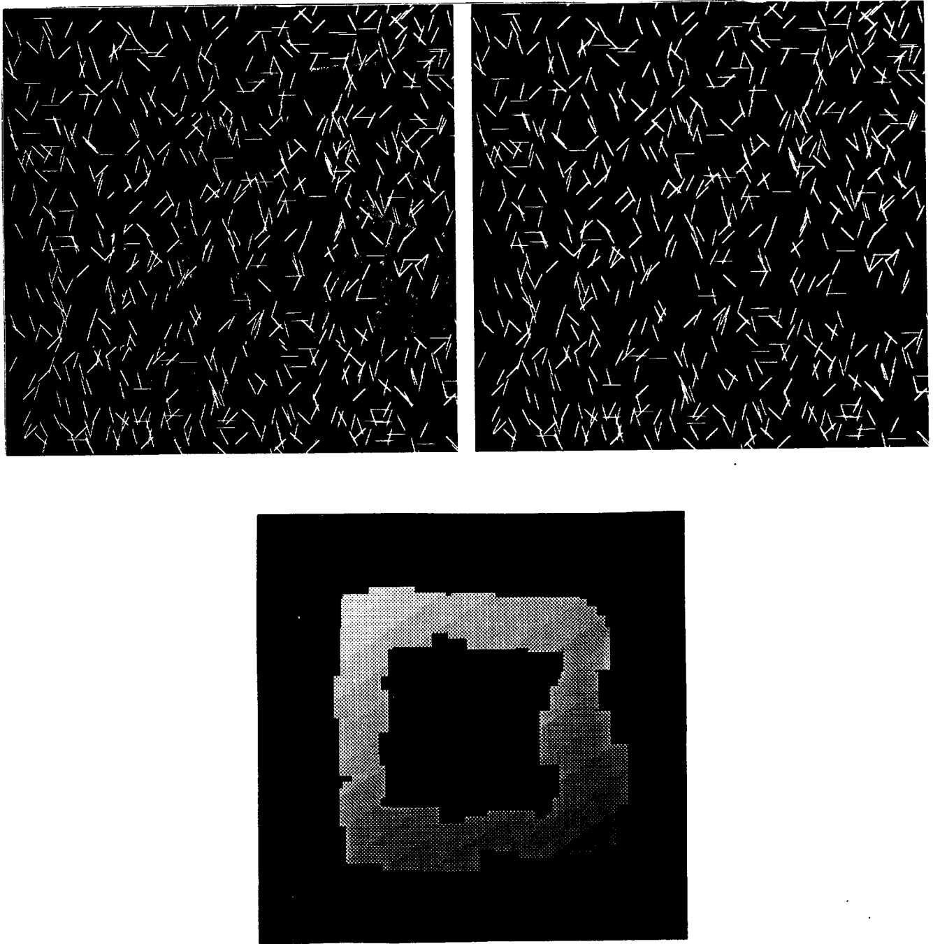
Figure 3.4: Results of a computer experiment with the proposed method for recovering the discontinuities of curved surfaces. The top half of the figure displays a random line stereogram corresponding to the input disparity information. The disparity corresponds to a central planar region that has been rotated about an oblique axis by < 45^\circ . The bottom half of the figure shows the recovered regions of discontinuity. The recovered depth from the viewer is displayed in terms of grey levels with black the furthest and white the closest.
