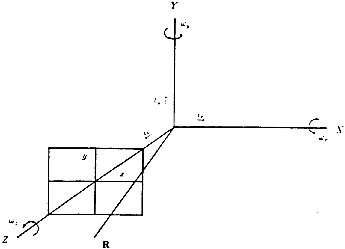
Figure 2.1: A general infinitesimal change of coordinates is composed of a translation \mathbf{T} = (t_x, t_y, t_z) and a rotation \mathbf{\Omega} = (\omega_x, \omega_y, \omega_z) . A point \mathbf{R} = (X, Y, Z) undergoes perspective projection onto a plane located at Z = 1 .
